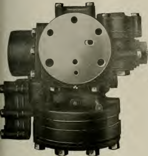
AUXILIARY RESERVOIR SIDE. TYPE S-2 TRIPLE VALVE
